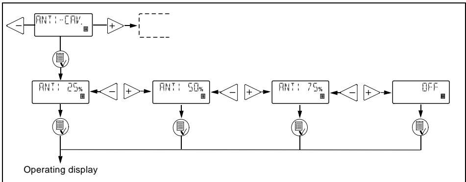
Fig. 6 Anti-cavitation function
