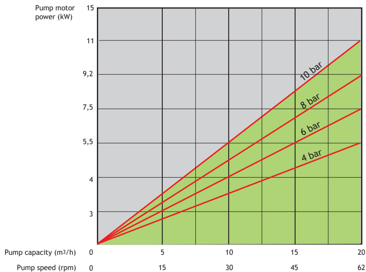
LPP-T65 CAPACITY CHART, CONTINUOUS DUTY UP TO 95 °C
