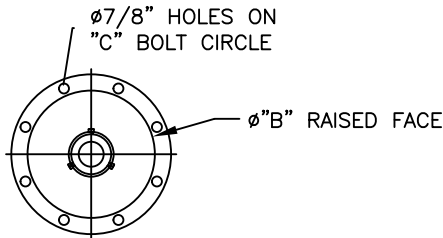
MOUNTING FLANGE ORIENTATION
