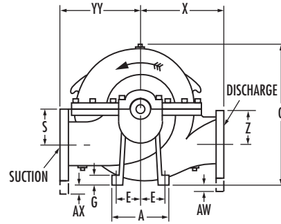
RIGHT-HAND ROTATION
