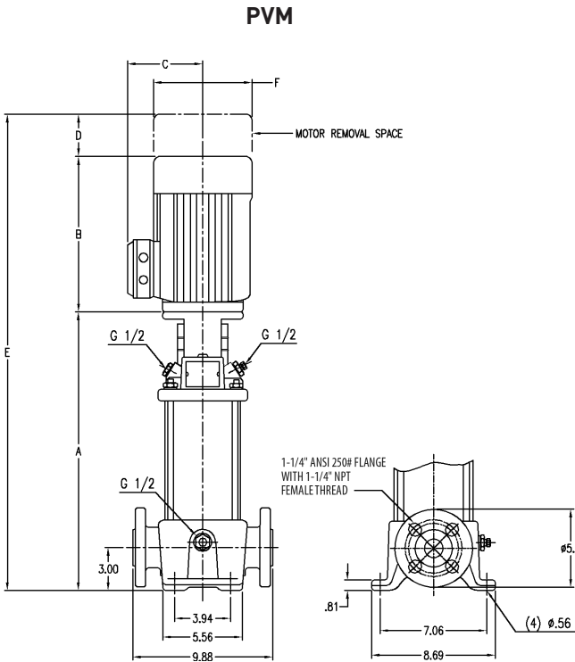
Dual 1-1/4" NPT / 1-1/4" ANSI 250# Flanges
