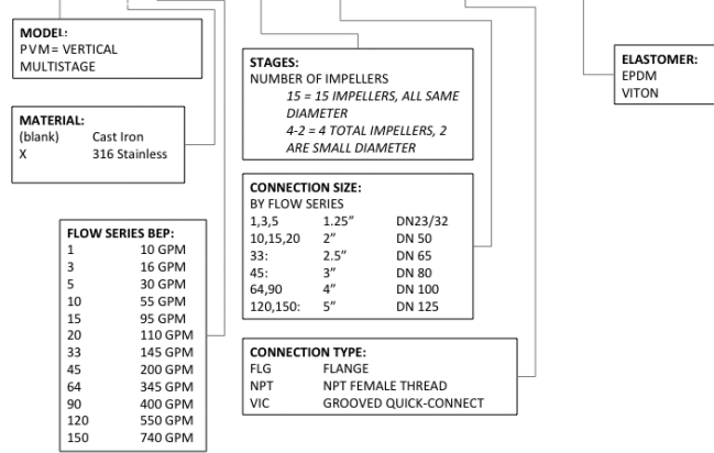
Figure 1 - Model Plate Information
