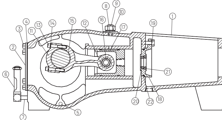
Power Frame Assembly; Connecting Rod, Crosshead & Wiper Box Assembly
