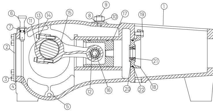
Power Frame Assembly; Connecting Rod, Crosshead & Wiper Box Assembly
