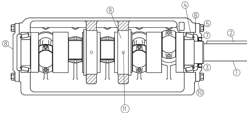
Crankshaft Assembly 2-3/4" Stroke; Right-Hand and Left-Hand Drive; Right-Hand Shown
