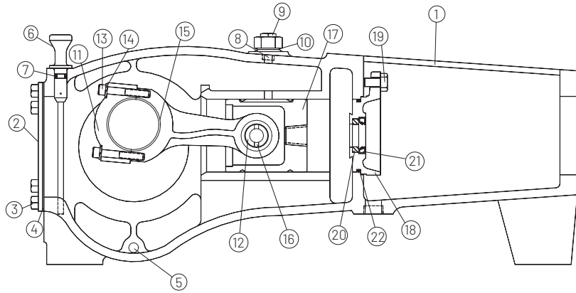
Power Frame Assembly; Connecting Rod, Crosshead & Wiper Box Assembly
