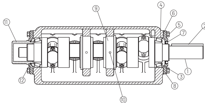
Crankshaft Assembly 2-1/4" Stroke; Right-Hand and Left-Hand Drive; Right-Hand Shown
