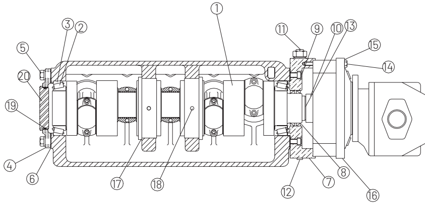
Crankshaft Assembly 2-3/4" Stroke; Auburn Planetary Gear #6
