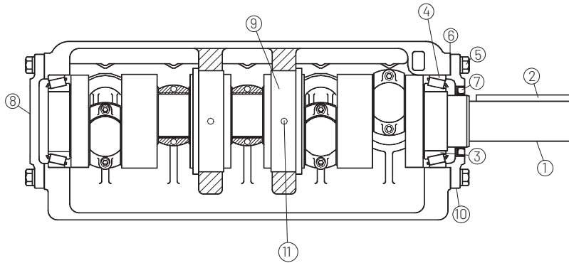
Crankshaft Assembly 2-1/4" Stroke; Right-Hand and Left-Hand Drive; Right-Hand Shown
