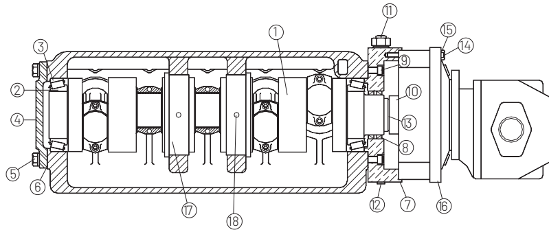
Crankshaft Assembly 2-3/4" Stroke; Auburn Planetary #8
