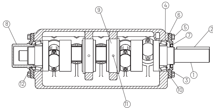
Crankshaft Assembly 2-3/4" Stroke; Right-Hand and Left-Hand Drive; Right-Hand Shown
